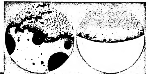
ABOVE TO LEFT —An ordinary weld between Iridium Tip and gold nib. Notice the many crater-like voids in the welded gold. This condition is responsible for tips snapping off. TO RIGHT —Parker Osmiridium tip, electrically fused to gold nib. Notice perfect, inseparable weld and complete absence of craters. Both views magnified 100 diameters.
